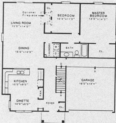
FIRST FLOOR 1298 SQ. FT.
