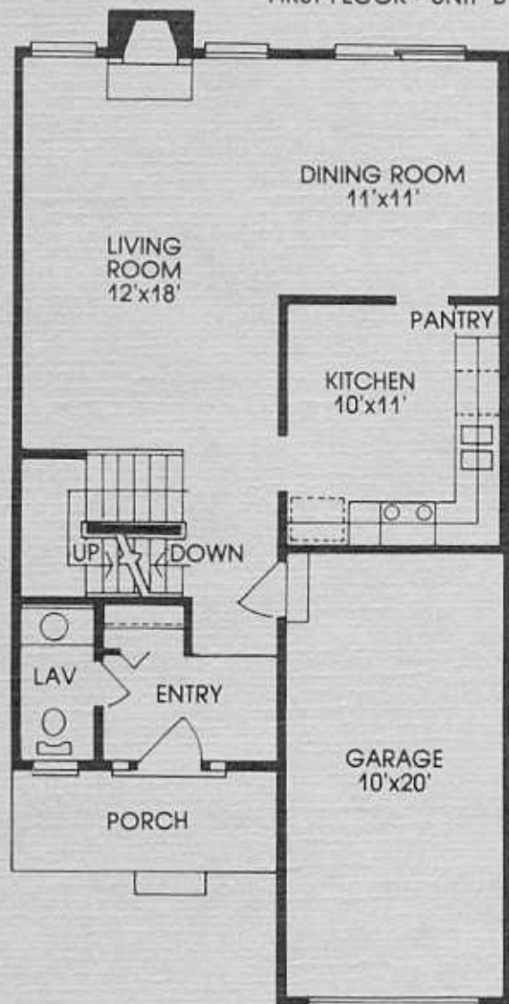
FIRST FLOOR - UNIT 'B'
